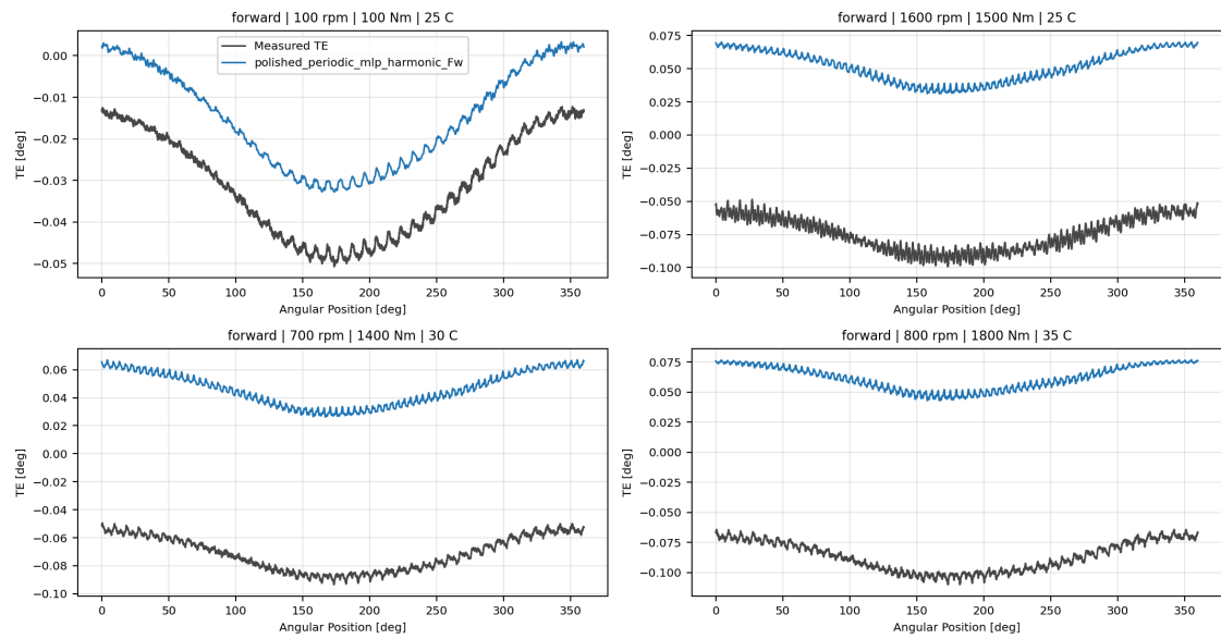
polished_periodic_mlp_harmonic_Fw measured-versus-predicted TE collage
