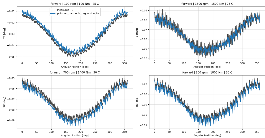
polished_harmonic_regression_Fw measured-versus-predicted TE collage
