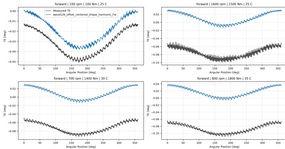
wave52b_offset_centered_shape_harmonic_Fw measured-versus-predicted TE collage
