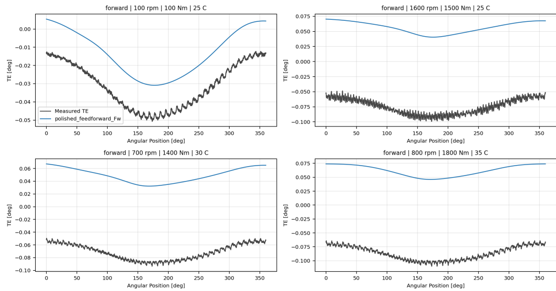
polished_feedforward_Fw measured-versus-predicted TE collage
