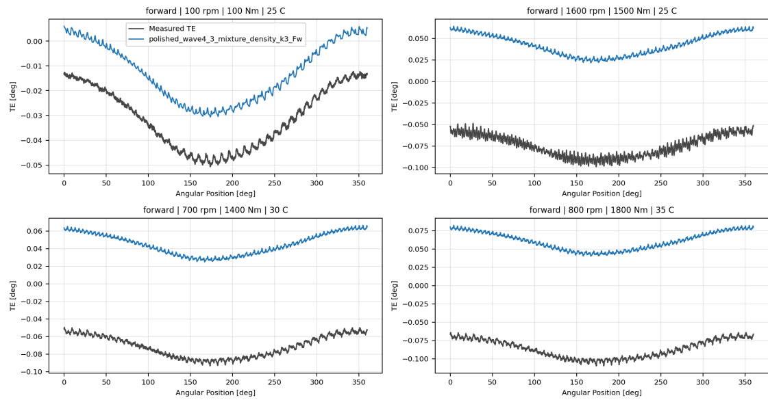
polished_wave4_3_mixture_density_k3_Fw measured-versus-predicted TE collage
