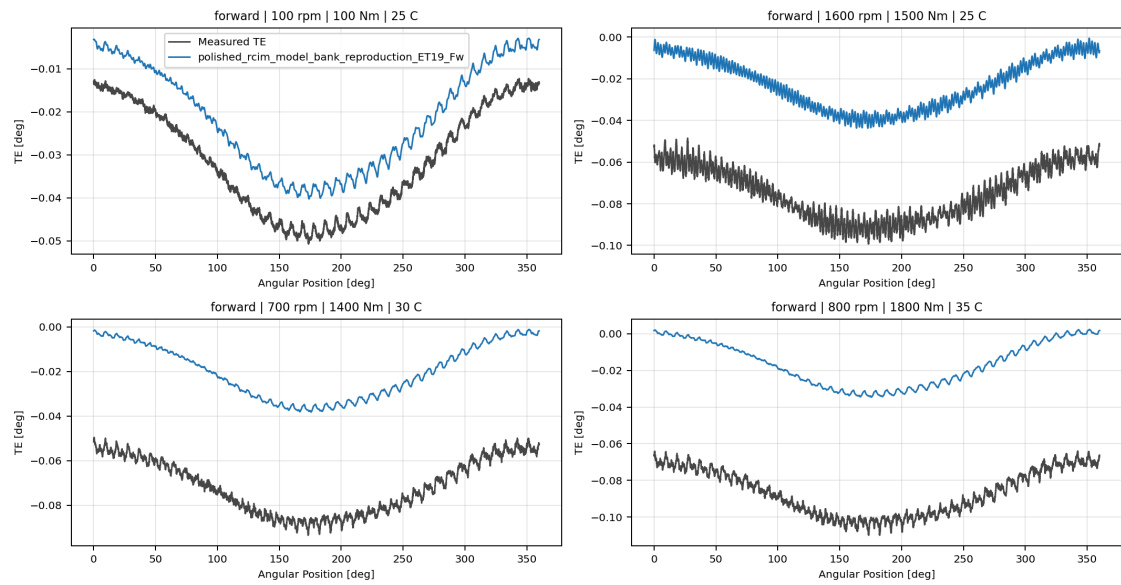
polished_rcim_model_bank_reproduction_ET19_Fw measured-versus-predicted TE collage
