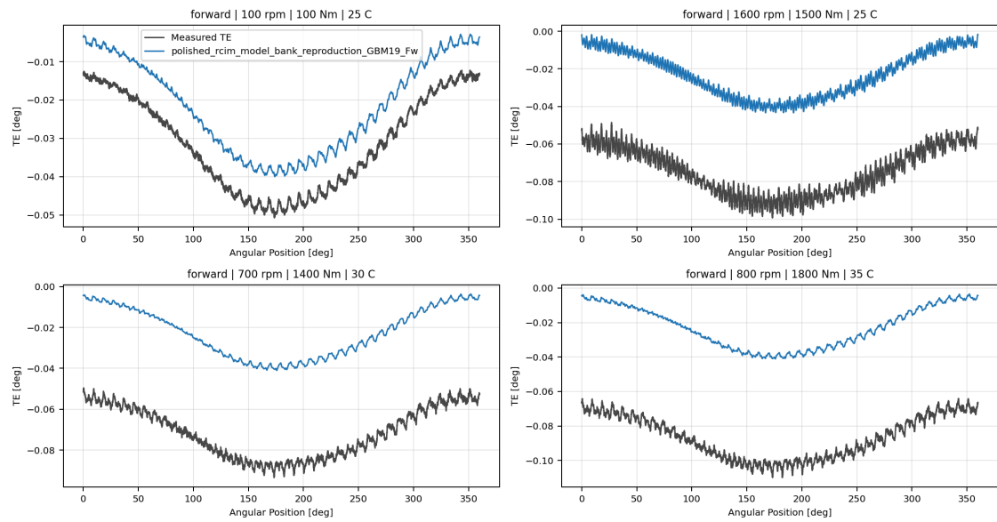
polished_rcim_model_bank_reproduction_GBM19_Fw measured-versus-predicted TE collage
