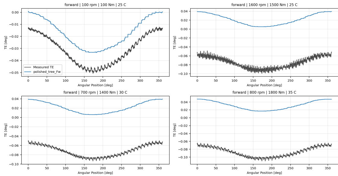
polished_tree_Fw measured-versus-predicted TE collage
