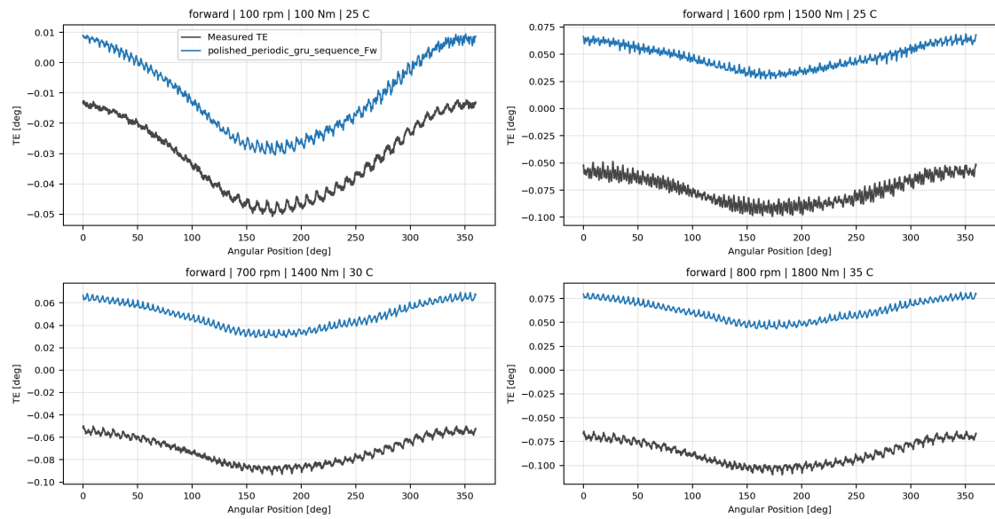
polished_periodic_gru_sequence_Fw measured-versus-predicted TE collage
